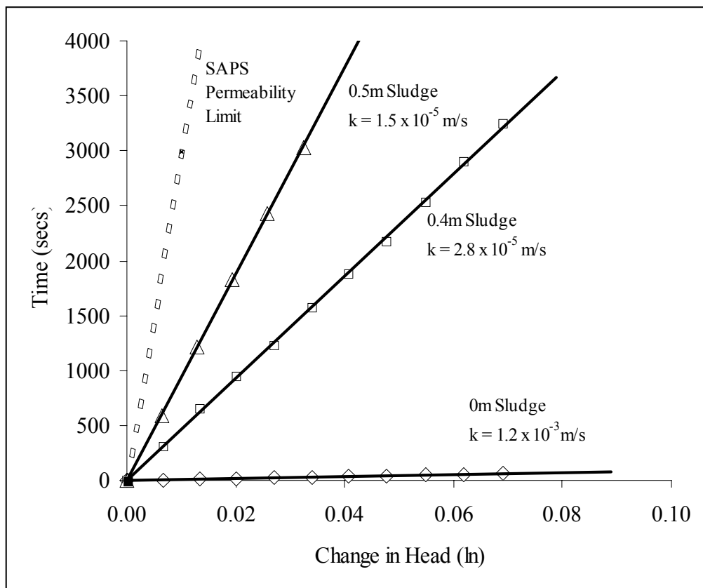
Figure 3. Variation of vertical permeability with ochre depth
